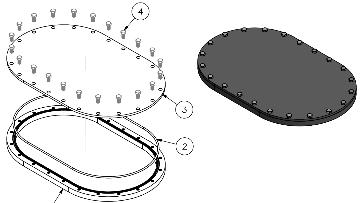
3D-IMPRESSION - EXPLODED VIEW
